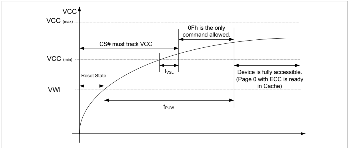
Figure 34 Power-On Timing
