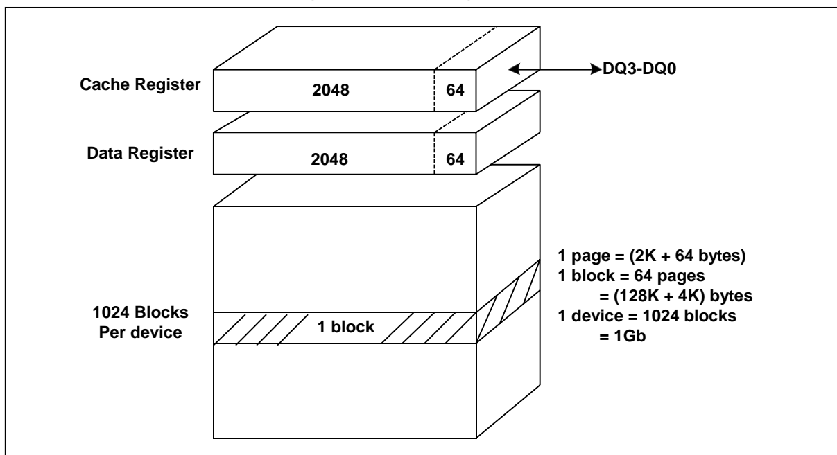
Figure 4 Array Organization
