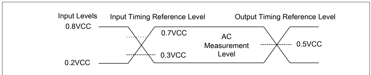
Figure 35 AC Measurement I/O Waveform
